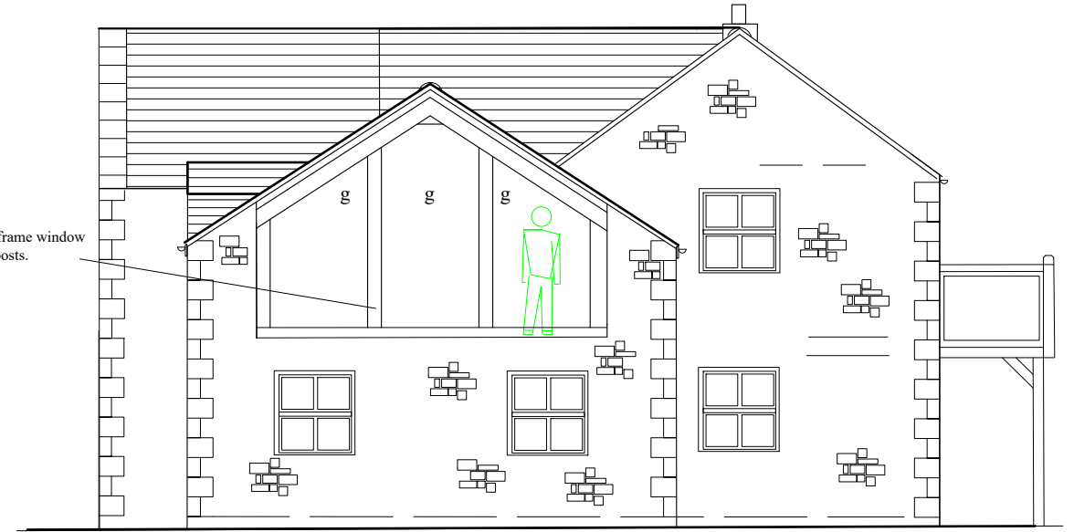
GABLE WEST ELEVATION
