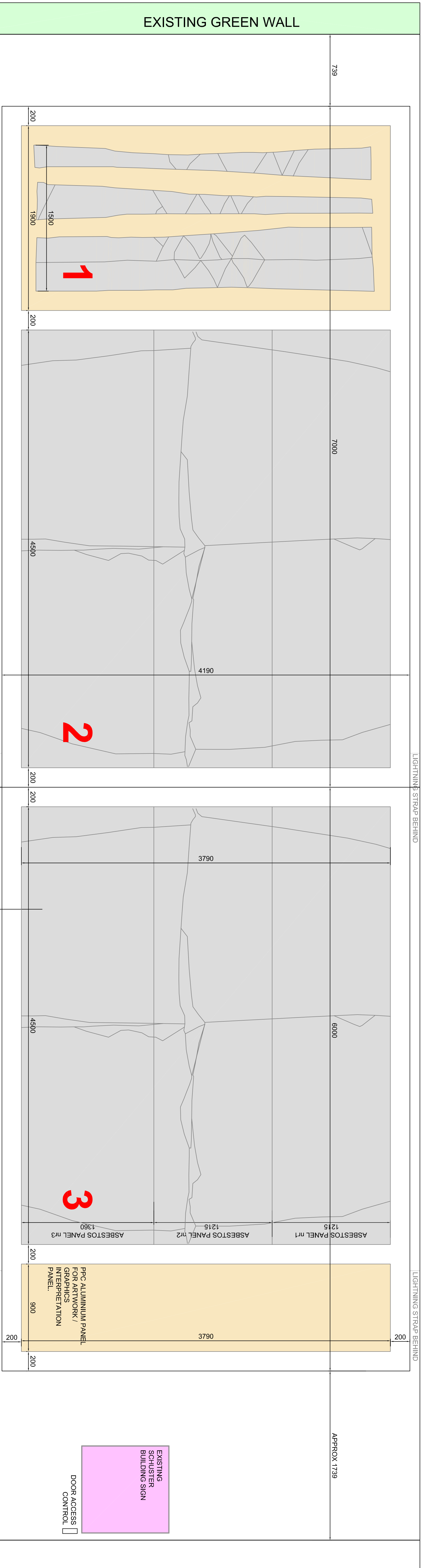
ELEVATION @1:20
