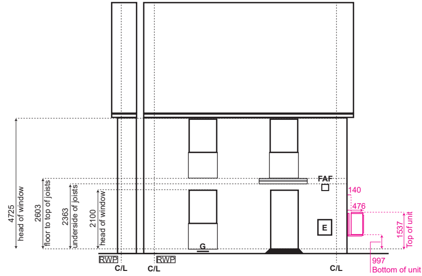
Front Elevation
