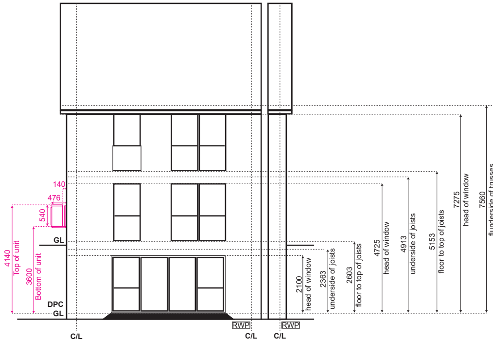
Rear Elevation
