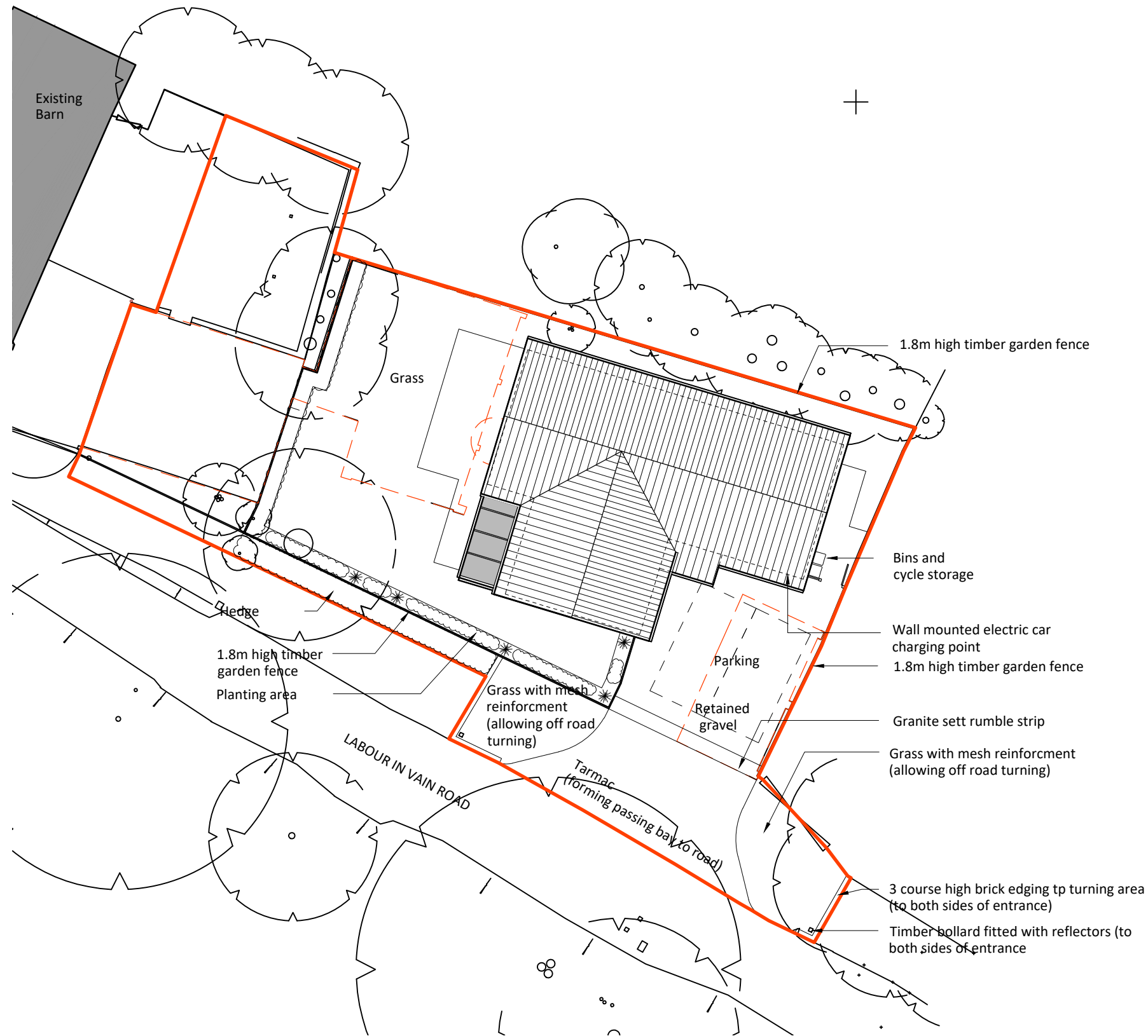
Proposed Block Plan 1:200
