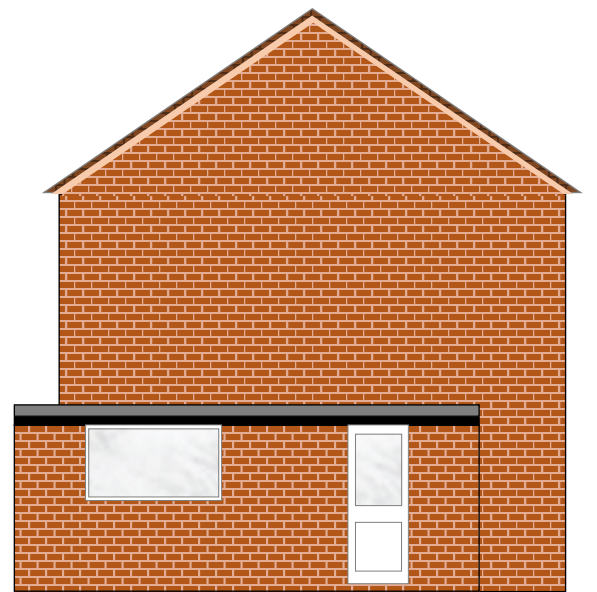
WEST SIDE ELEVATION
