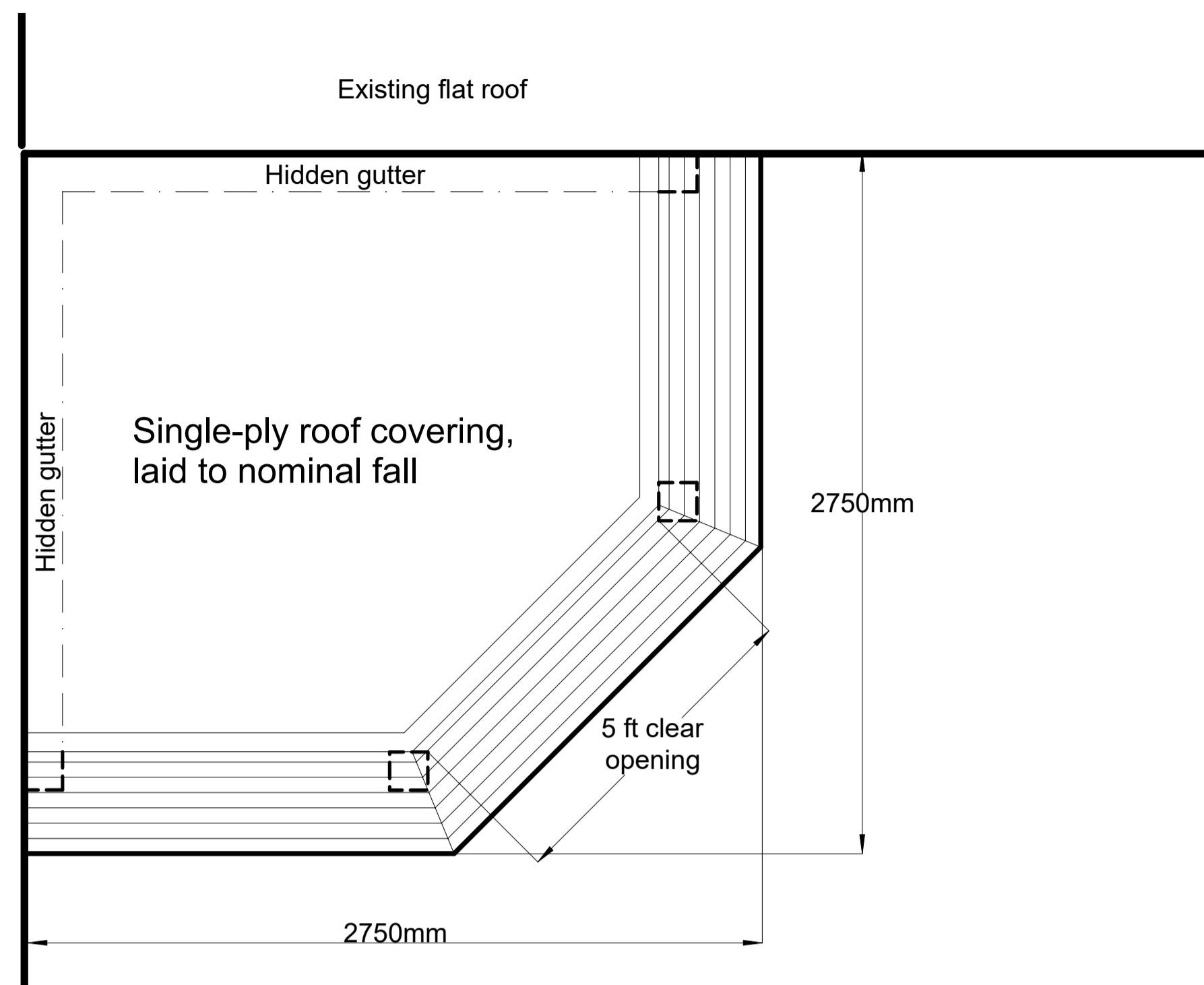
Proposed Porch - Plan - Scale 1:20
