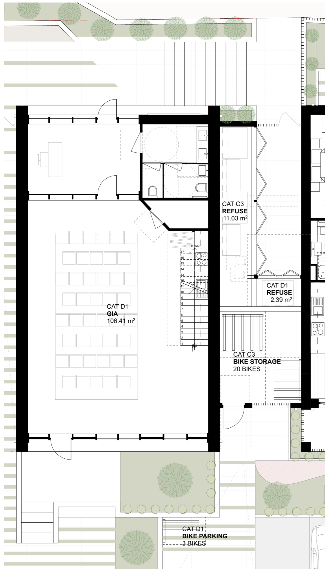
D1 Community Centre APPROVED PLAN 20 / 1469 / FUL Ground Floor GA Plan
