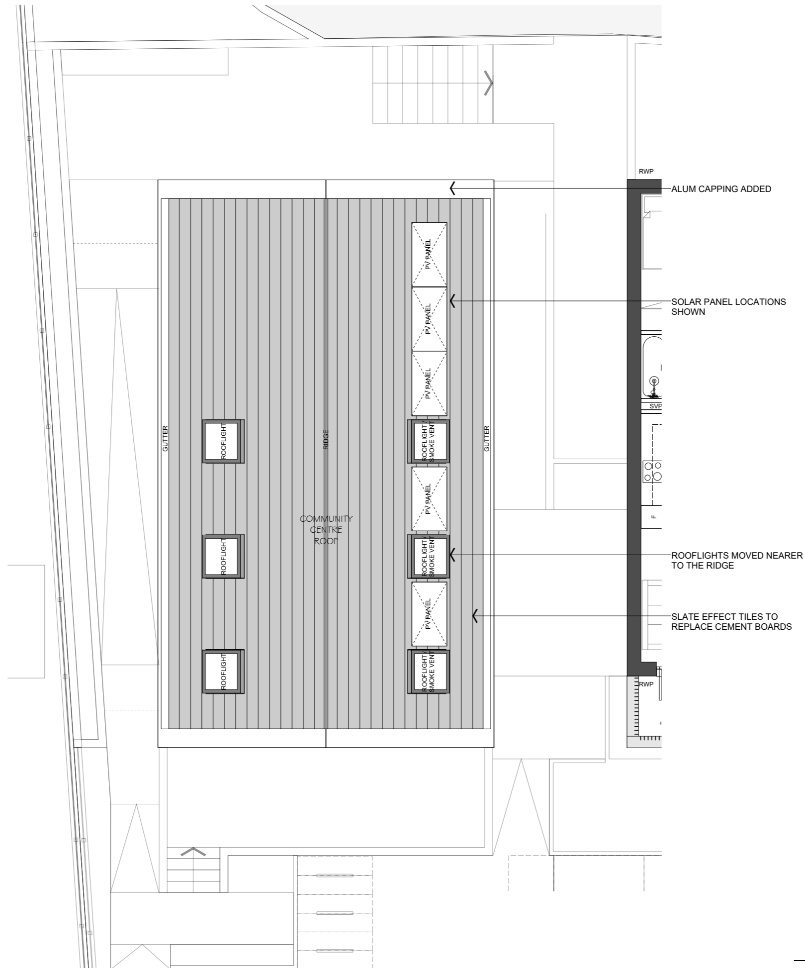
DI Community Centre PROPOSED MATERIAL CHANGE Roof Floor GA Plan
