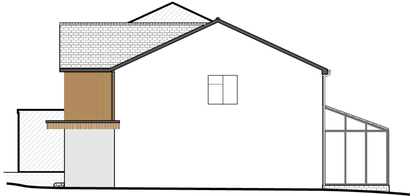
Right (west) elevation
