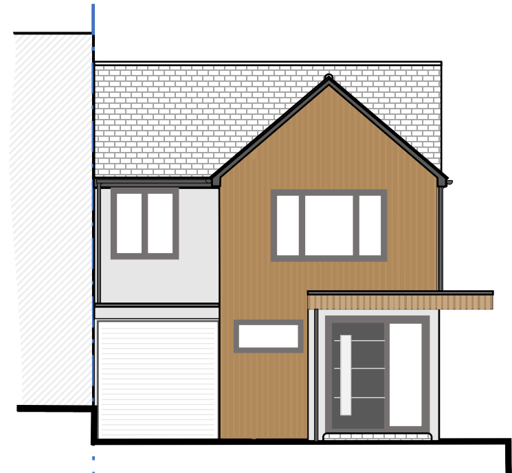
Front (north) elevation
