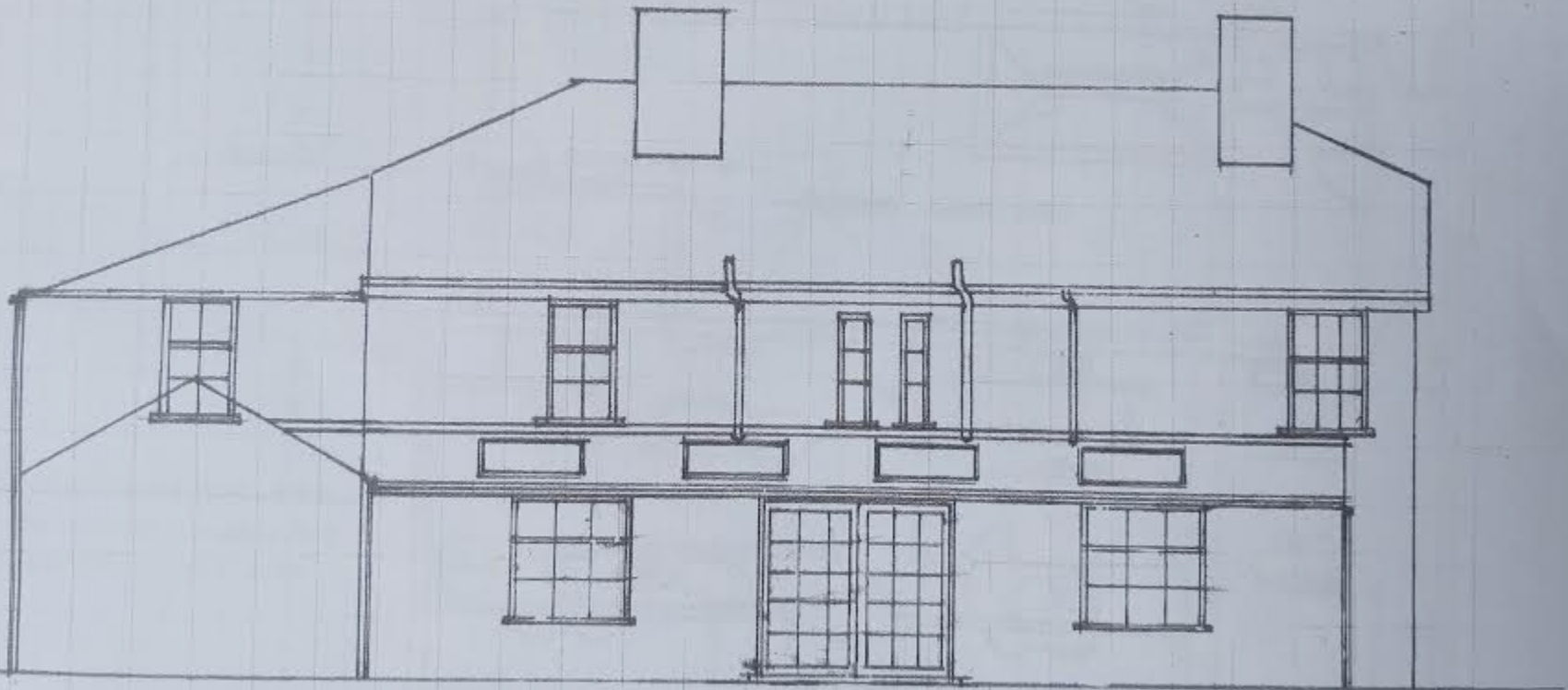
EAST FACE OF PROPOSED EXTENSION TO REAR OF PROPERTY FOR MR CUNNINGHAM 12 WELLS ROAD FAKENHAM
