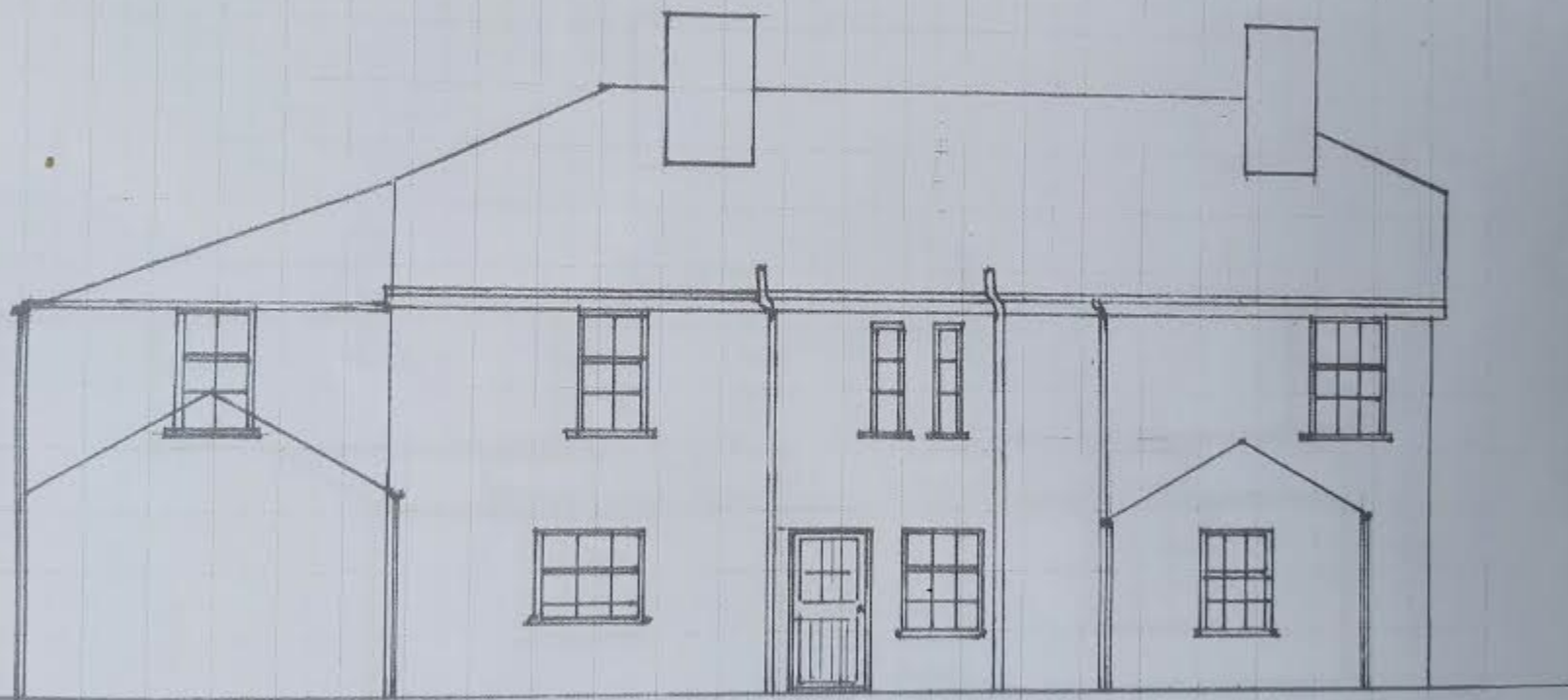
EAST FACE EXISTING VIEW FOR MR. C. CUNNINGHAM 12 WELLS ROAD FAREHAM SCALE 1:750
