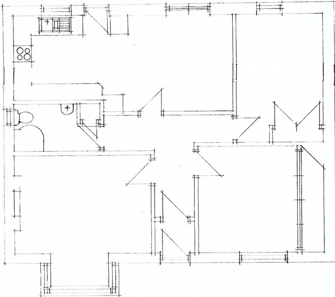
FLOOR PLAN AS EXISTING
