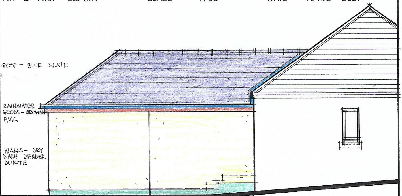
EAST ELEVATION
