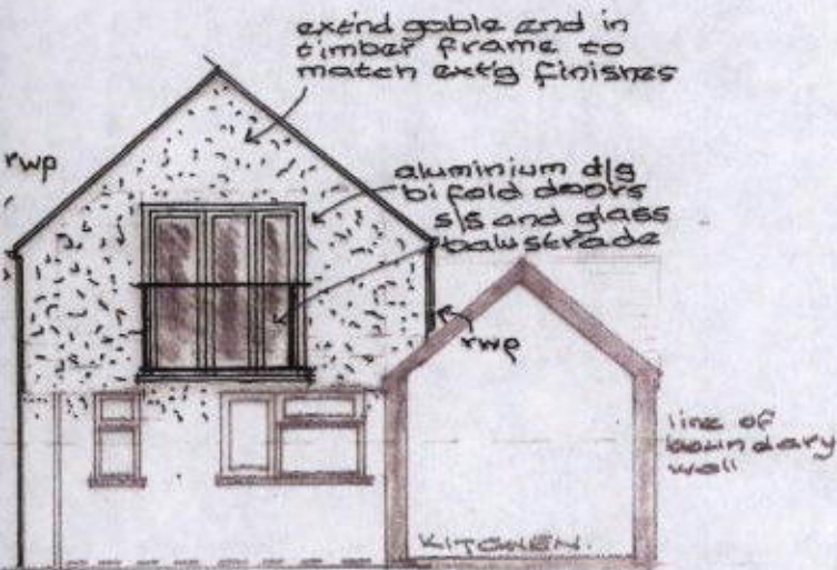
WEST ELEVATION
