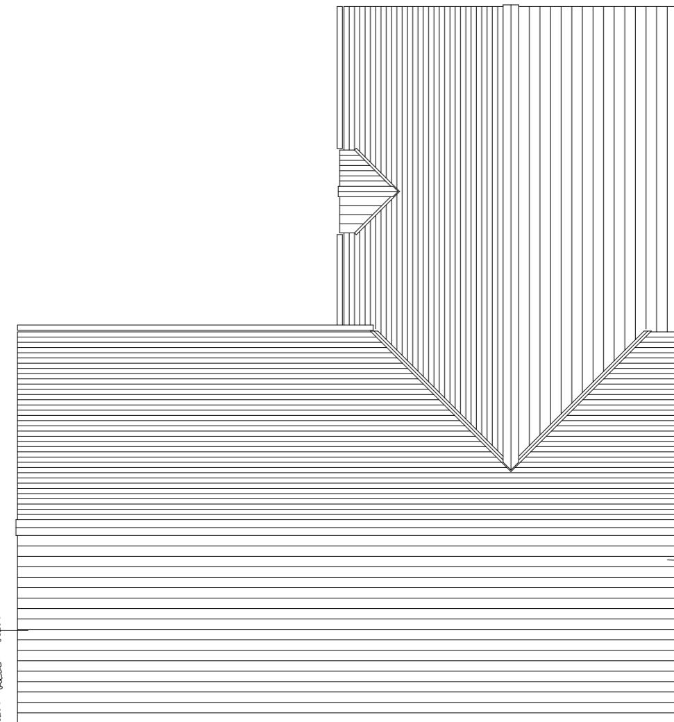
Roof Plan
