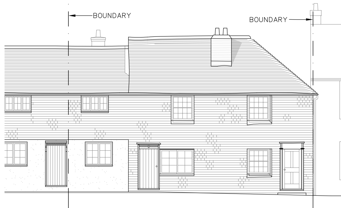
SOUTH (FRONT) ELEVATION
