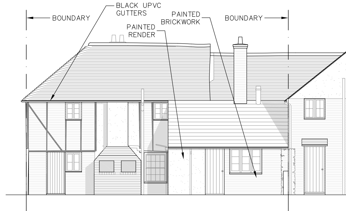
NORTH (REAR) ELEVATION
