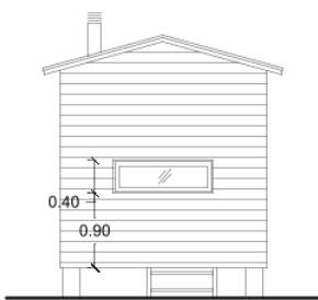
East Elevation
