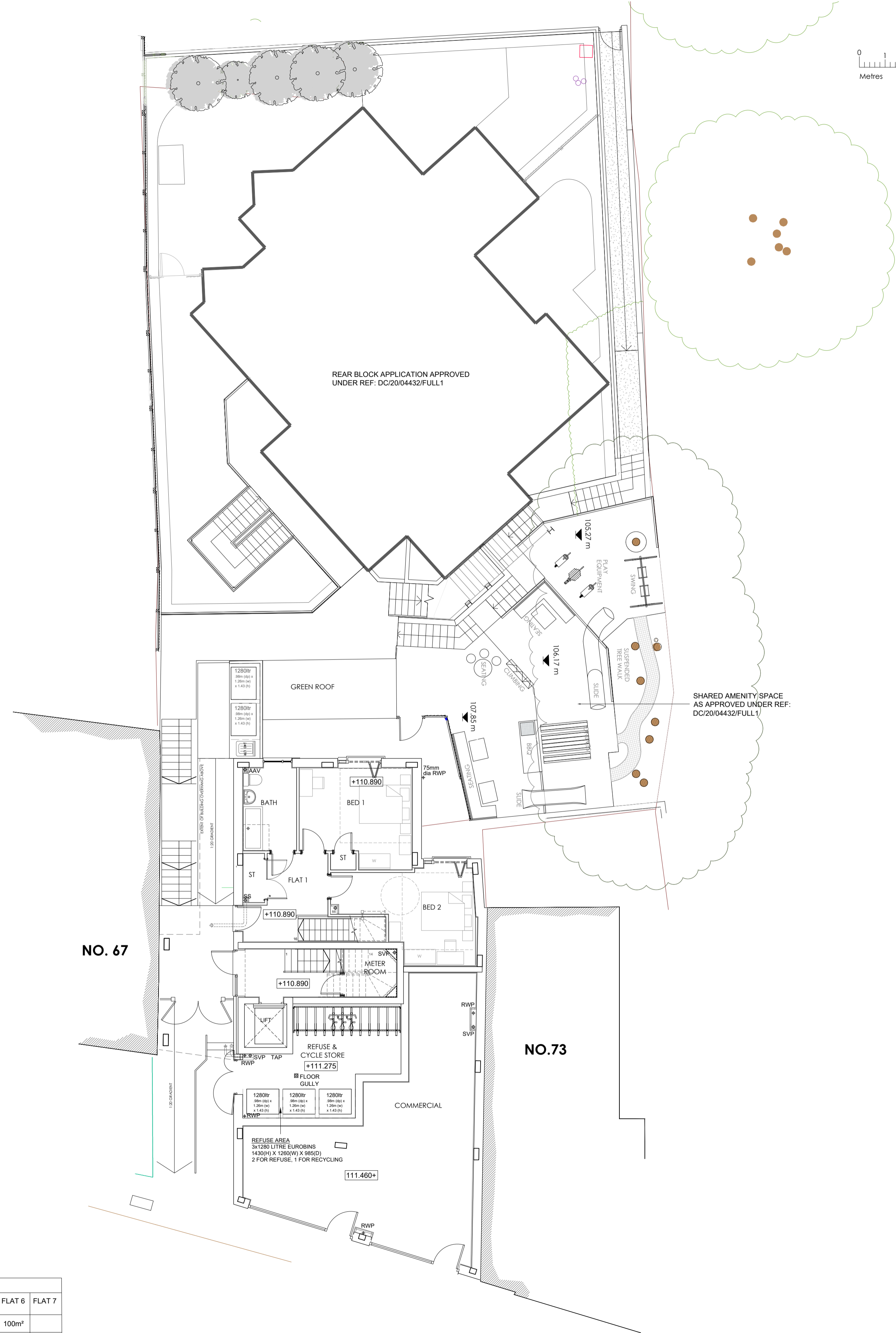
GROUND FLOOR PLAN SCALE 1:100
