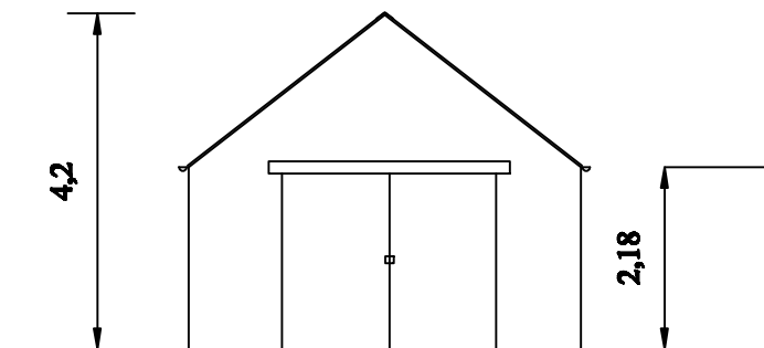
Existing East Elevation
