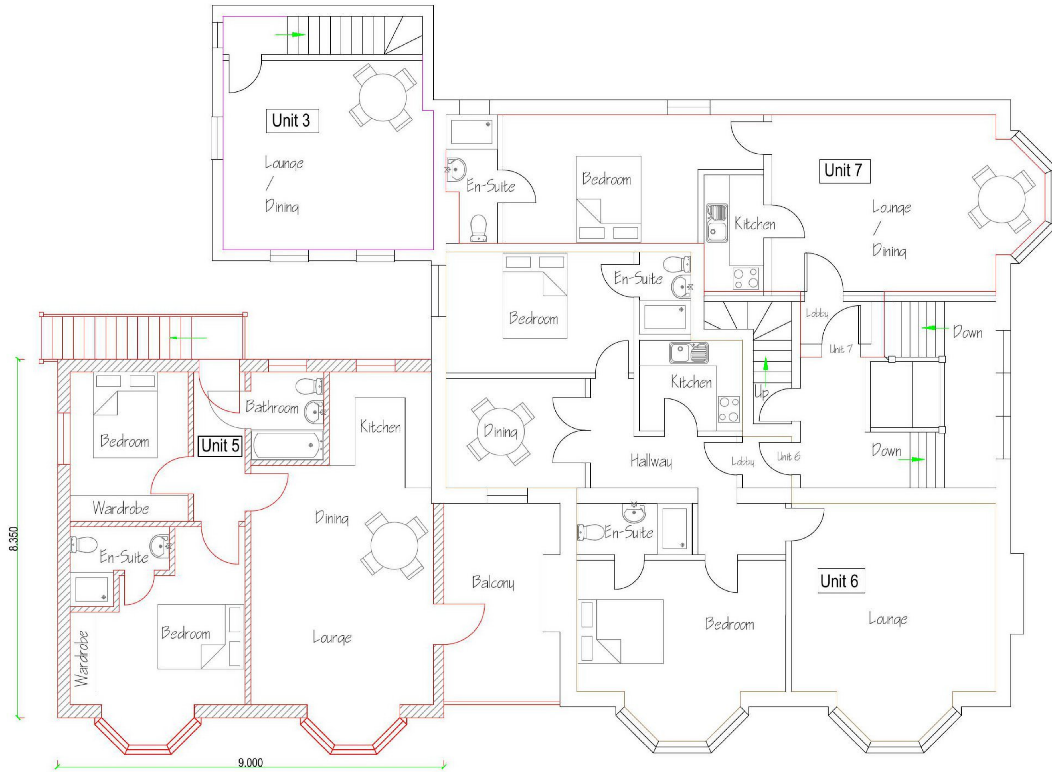
Proposed First Floor
