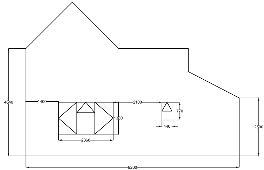
SIDE ELEVATION OF HOUSE - CURRENT
