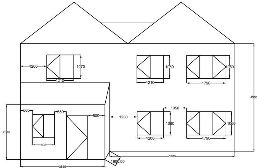
FRONT ELEVATION OF HOUSE - CURRENT
