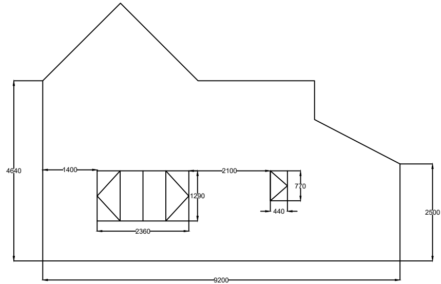
SIDE ELEVATION OF HOUSE - PROPOSED
