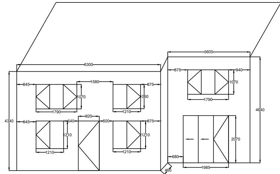
REAR ELEVATION OF HOUSE - PROPOSED (EXTENSION CONSERVATORY NOT INCLUDED IN DRAWING AS NO CHANGES ARE BEING DONE AND ENABLES EXPOSURE OF INTERNAL WINDOWS)
