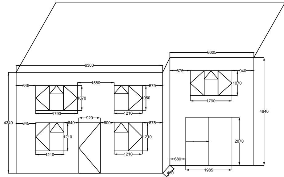
REAR ELEVATION OF HOUSE - CURRENT (EXTENSION CONSERVATORY NOT INCLUDED IN DRAWING AS NO CHANGES ARE BEING DONE AND ENABLES EXPOSURE OF INTERNAL WINDOWS)
