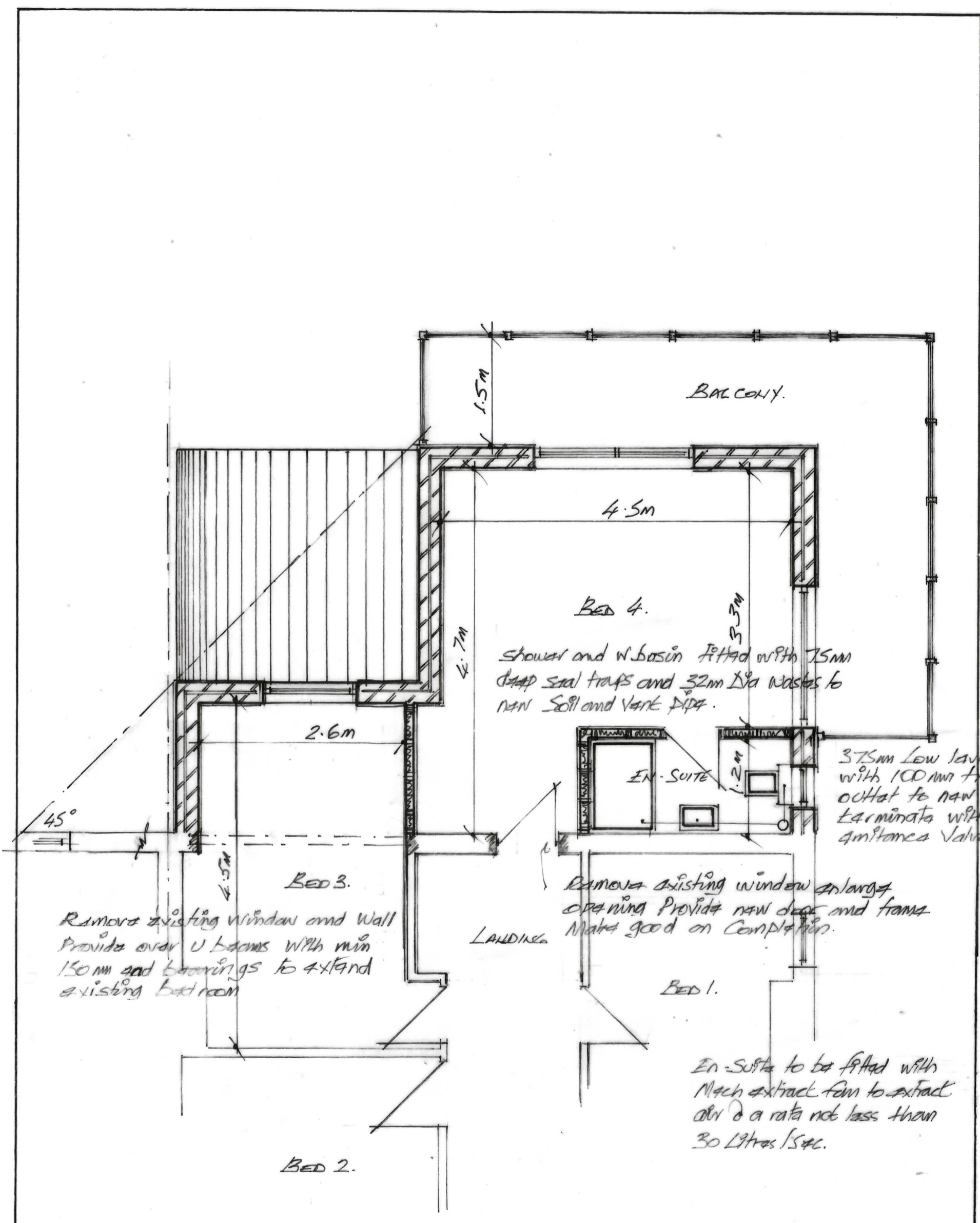
PROP F. FLOOR PLAN.
