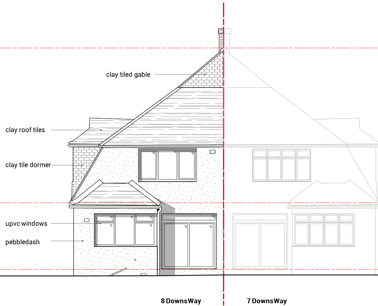
2 - Existing - West Elevation
