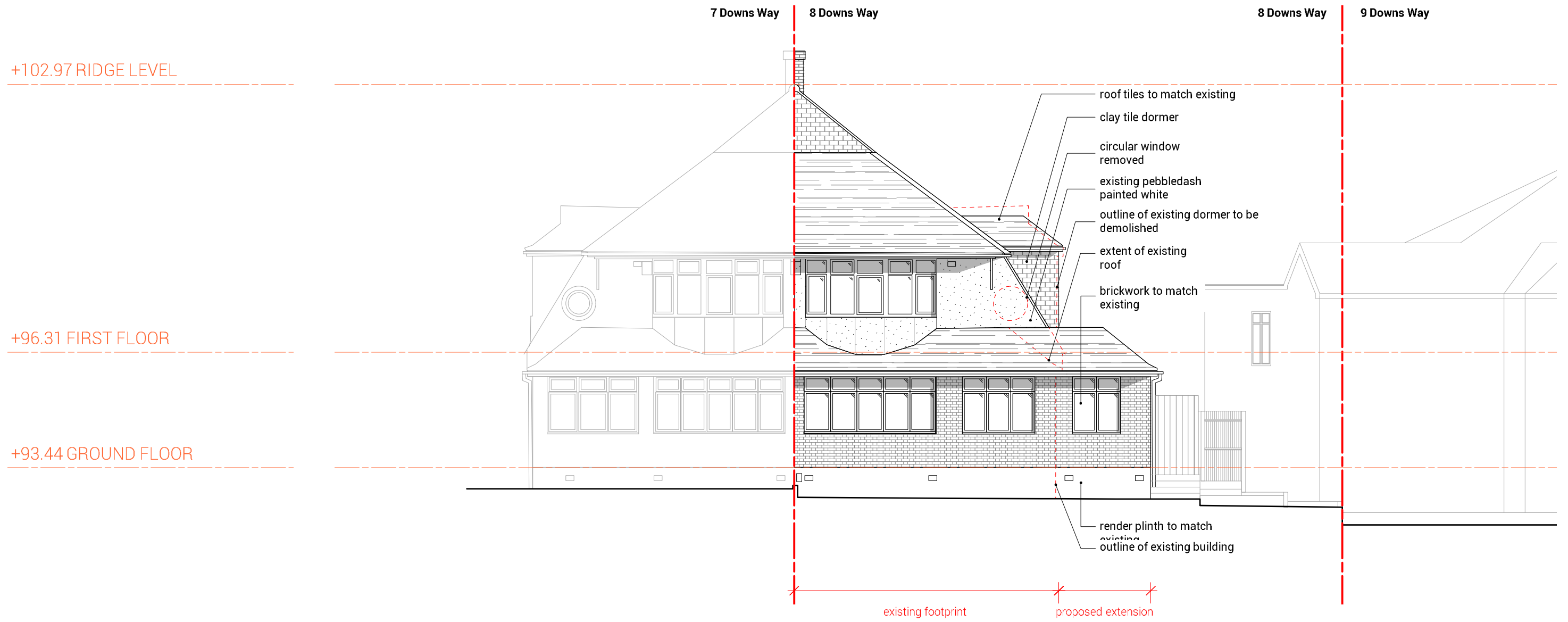
1 - Proposed - East Elevation
