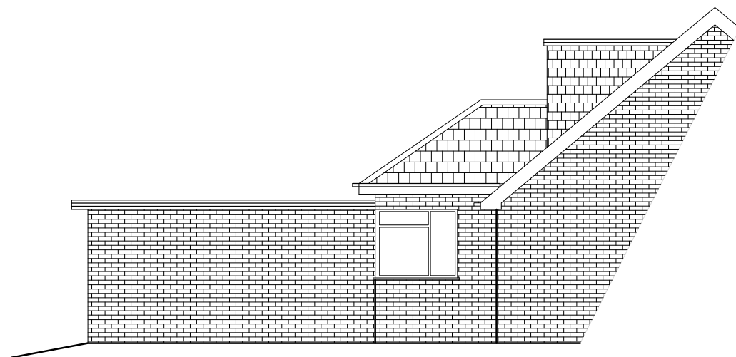
Part South West Elevation Existing
