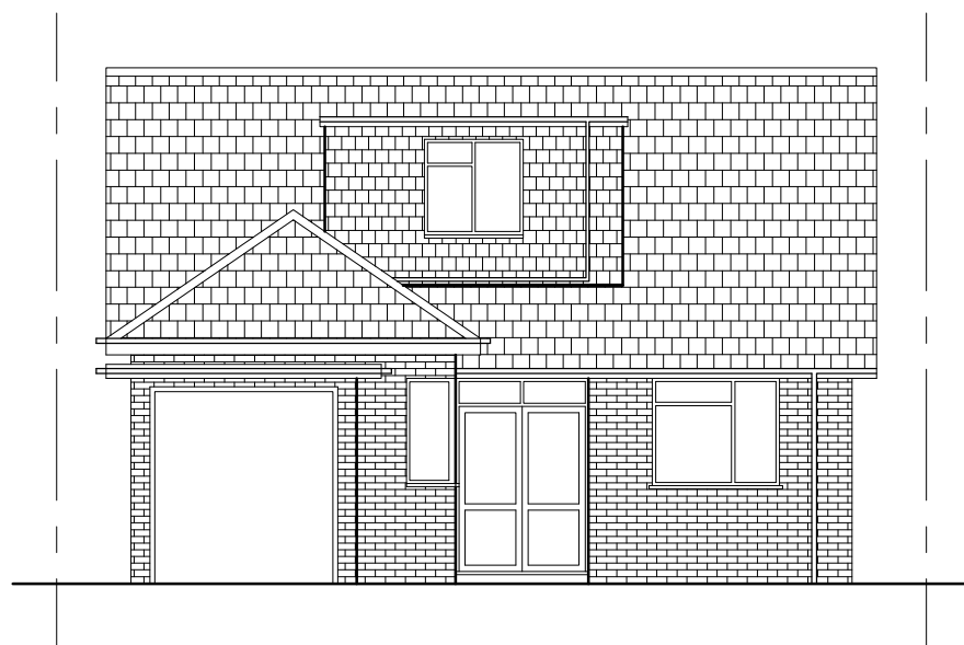
Front Elevation Existing
