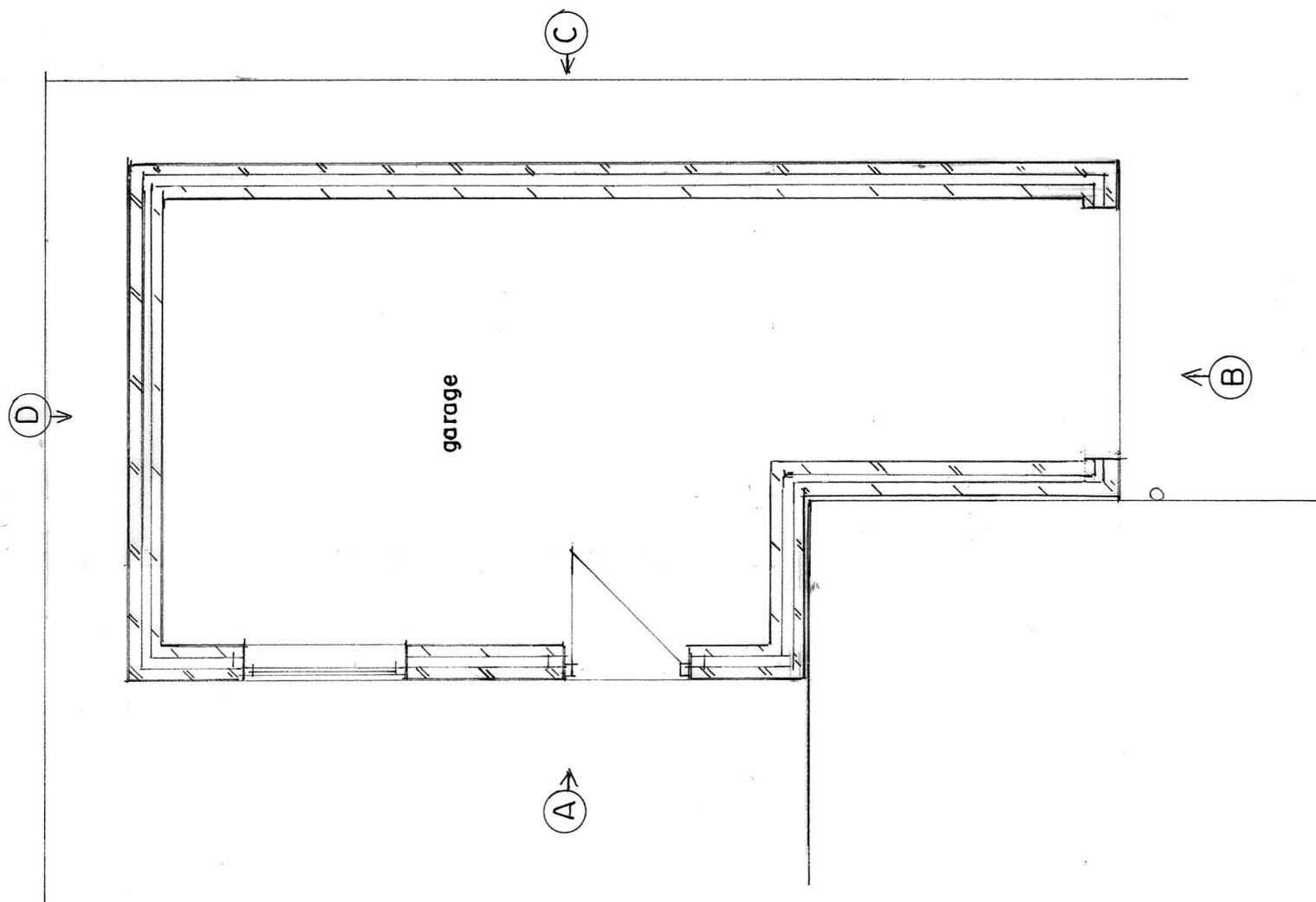
PLAN (PROPOSED)
