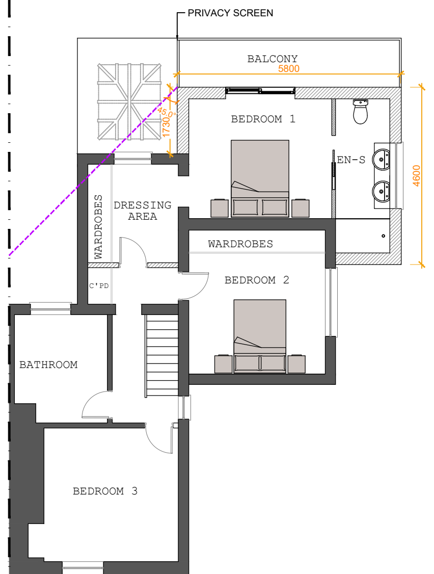
PROPOSED FIRST FLOORPLAN 1:100 @ A3
