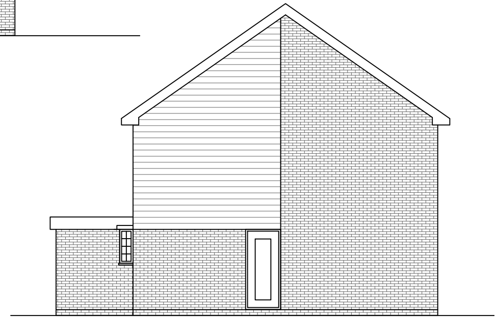
SIDE ELEVATION
