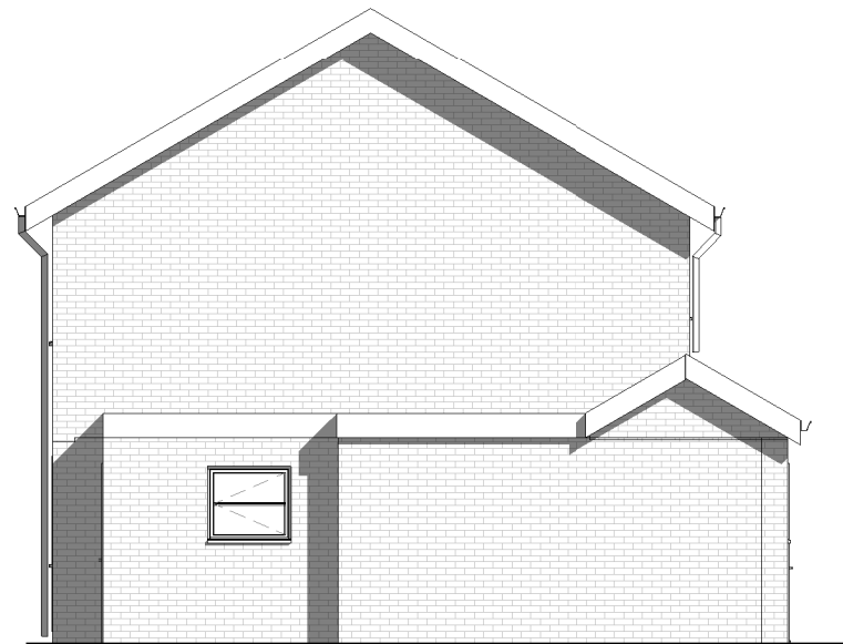
6 Proposed Side. Elevation 1 : 100
