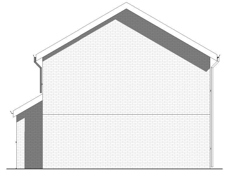
3 Proposed Side Elevation 1 : 100
