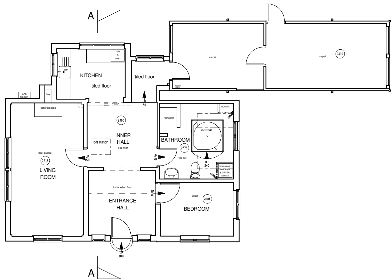
GROUND FLOOR LAYOUT PLAN
