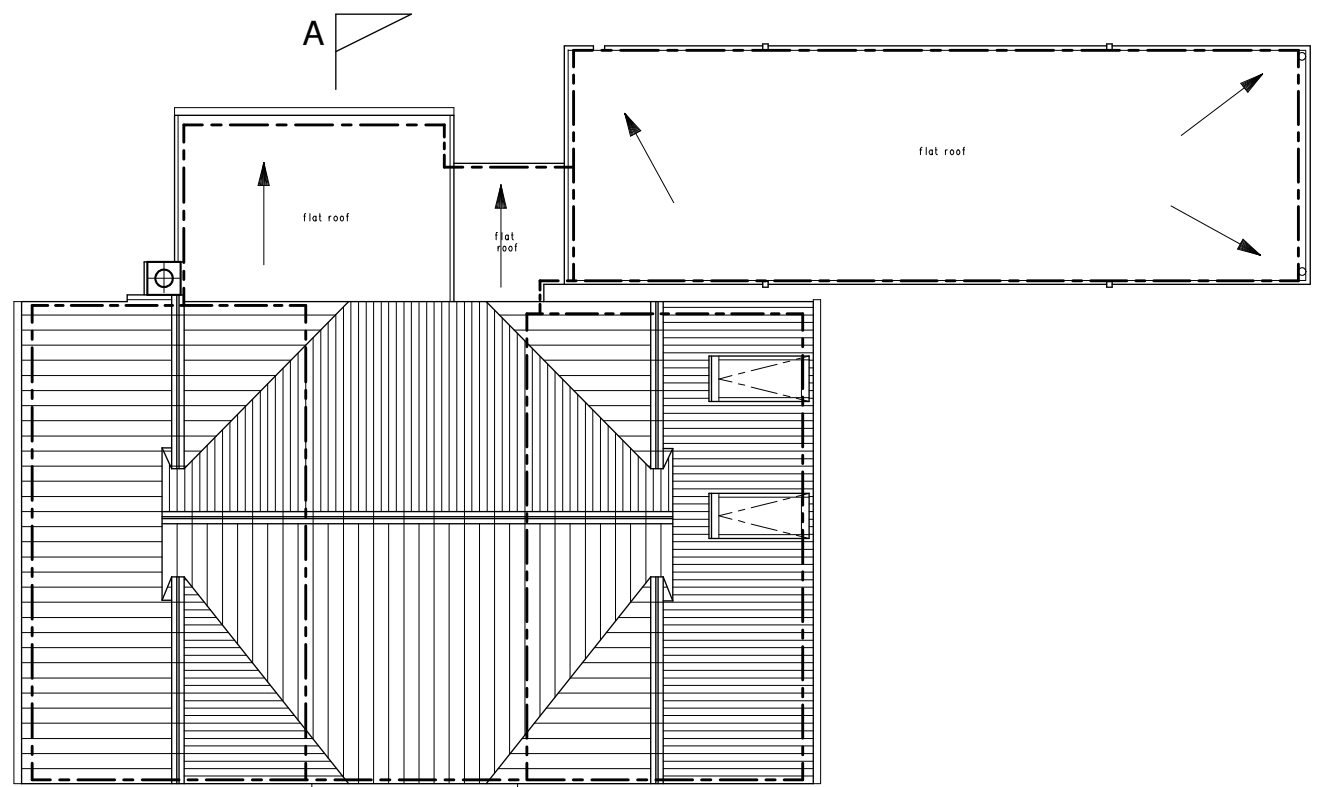
ROOF PLAN
