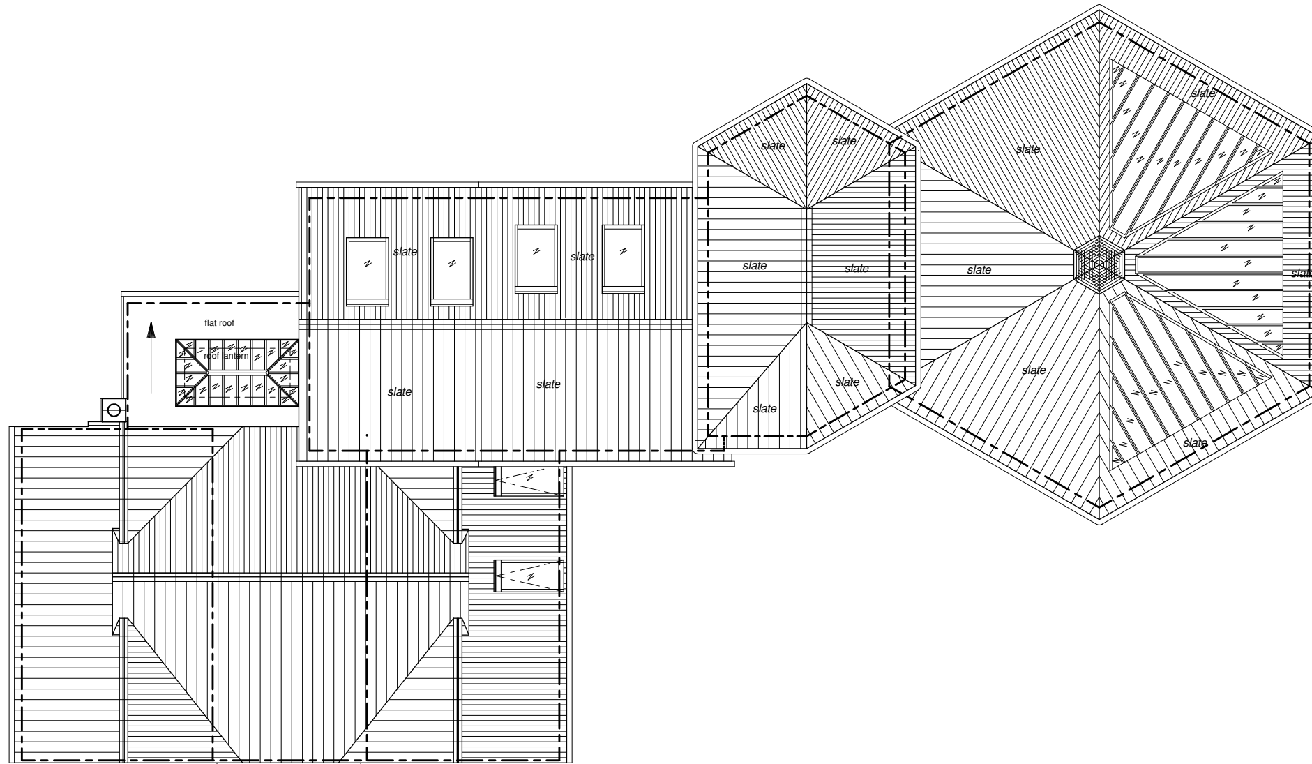
ROOF LAYOUT PLAN
