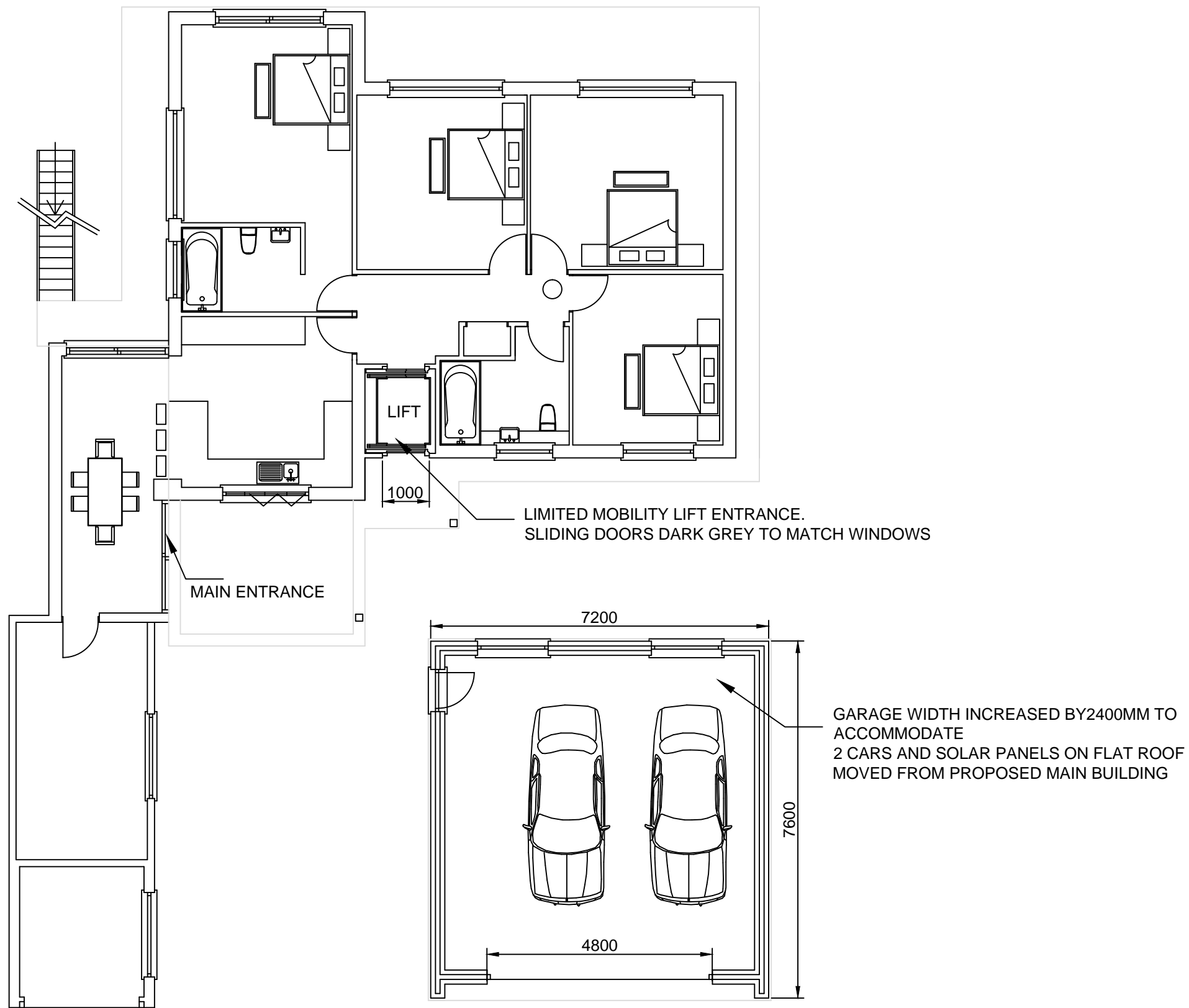
PROPOSED GROUND FLOOR PLAN AMENDMENT 1:100
