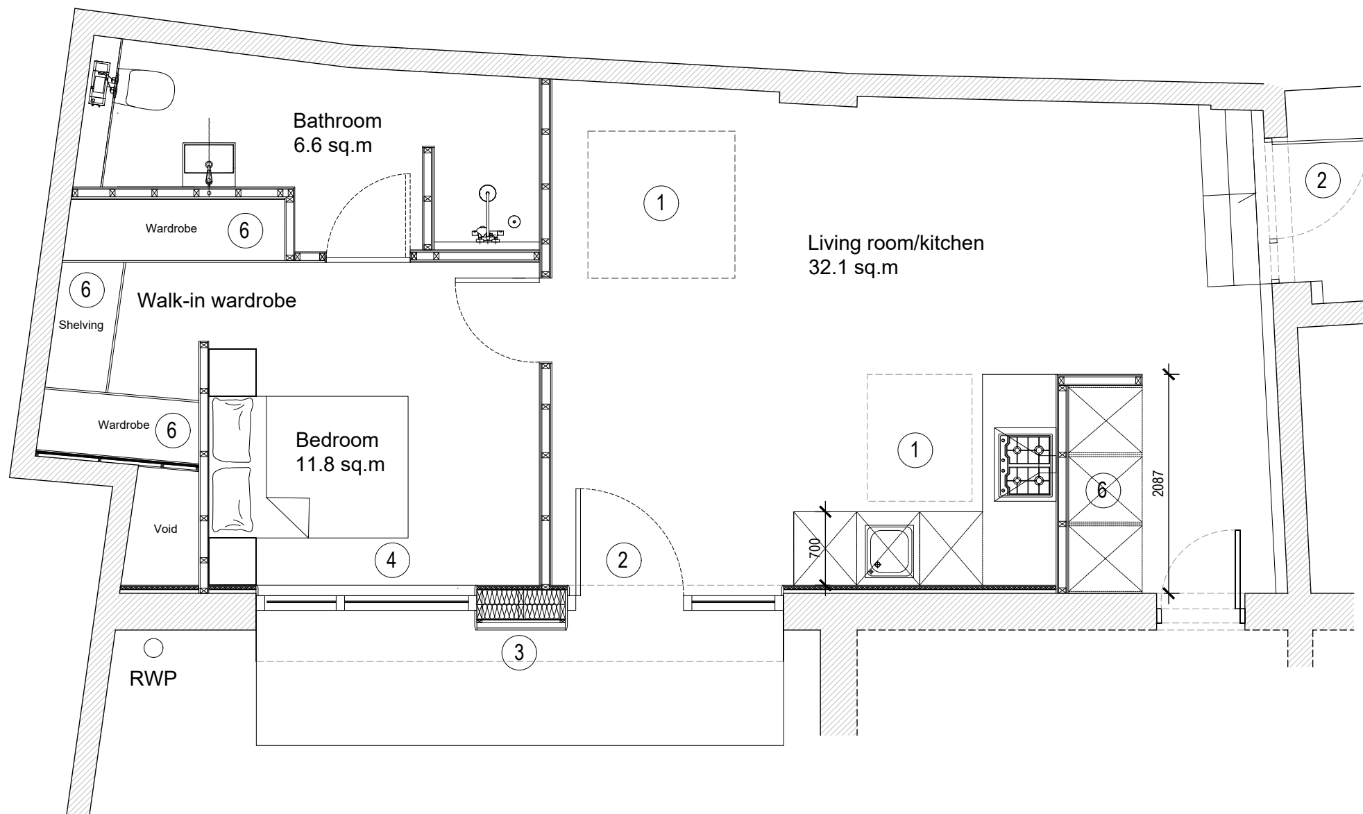
① Proposed Layout 1:50
