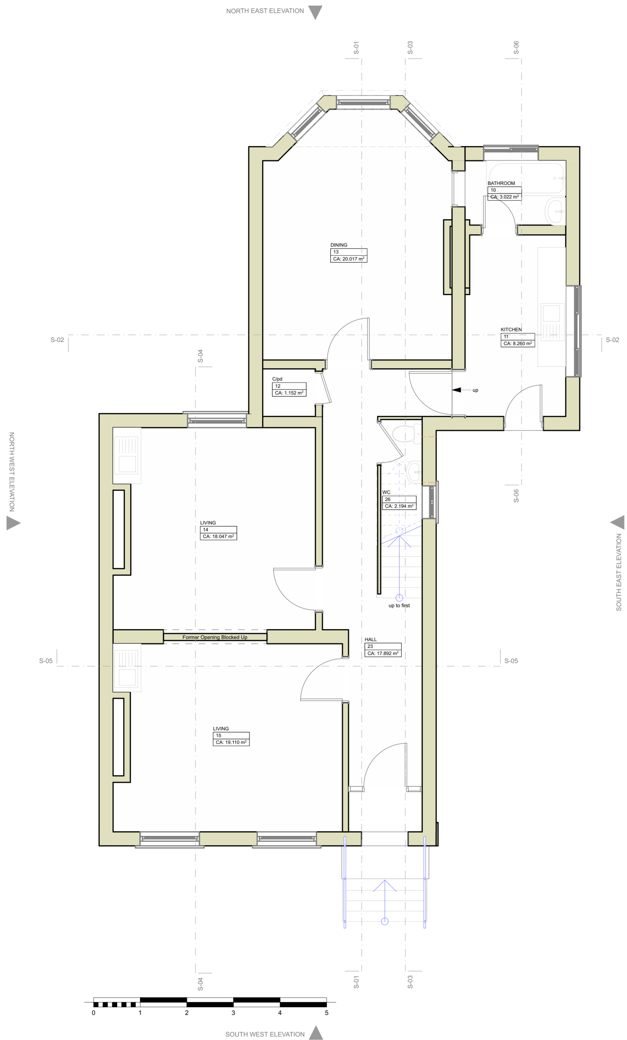
1 GF-Ground Floor 1:50
