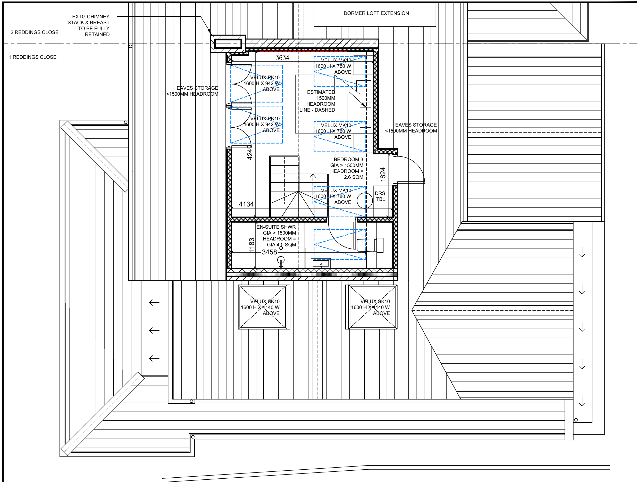
1 PROPOSED LOFT FLOOR PLAN 1:50
