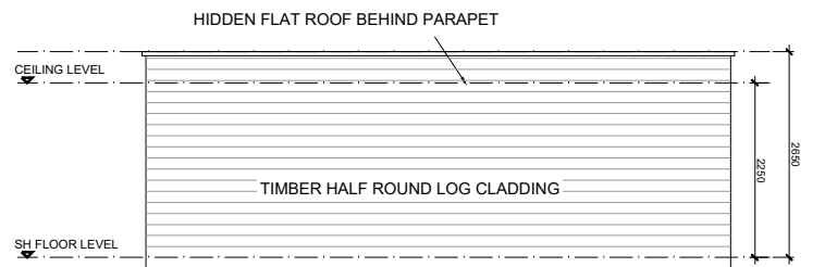
REAR ELEVATION AS PROPOSED
