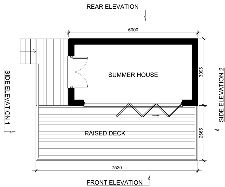
FLOOR PLAN AS PROPOSED
