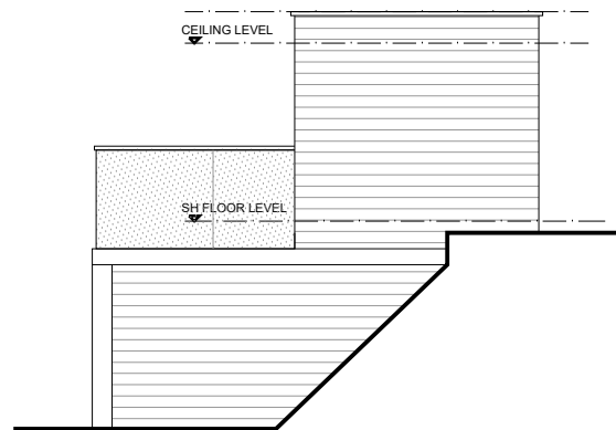
SIDE ELEVATION 2 AS PROPOSED
