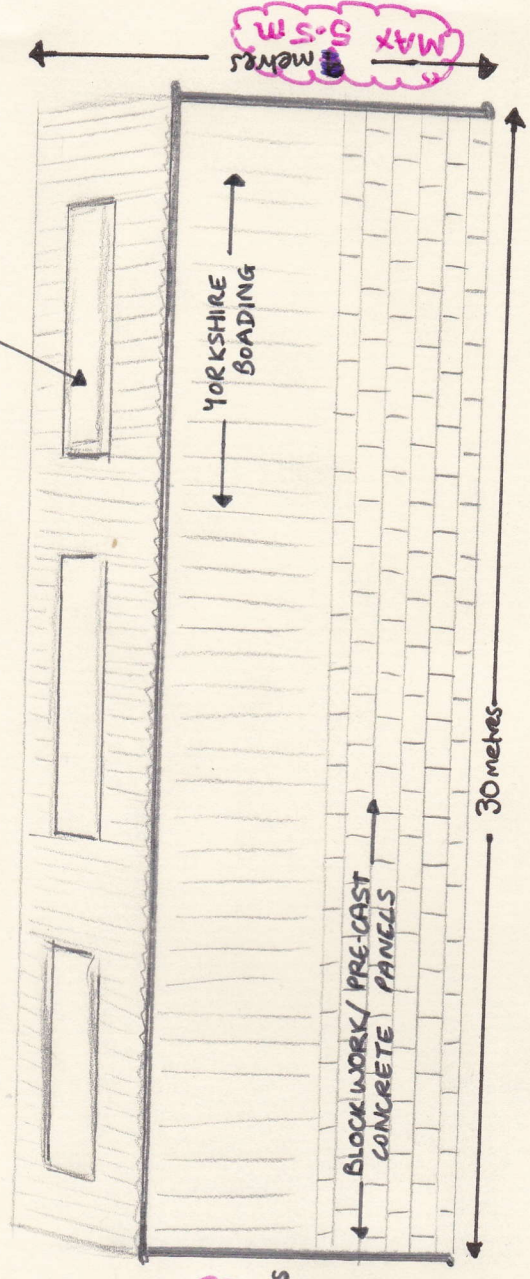
SOUTHERLY ELEVATION
