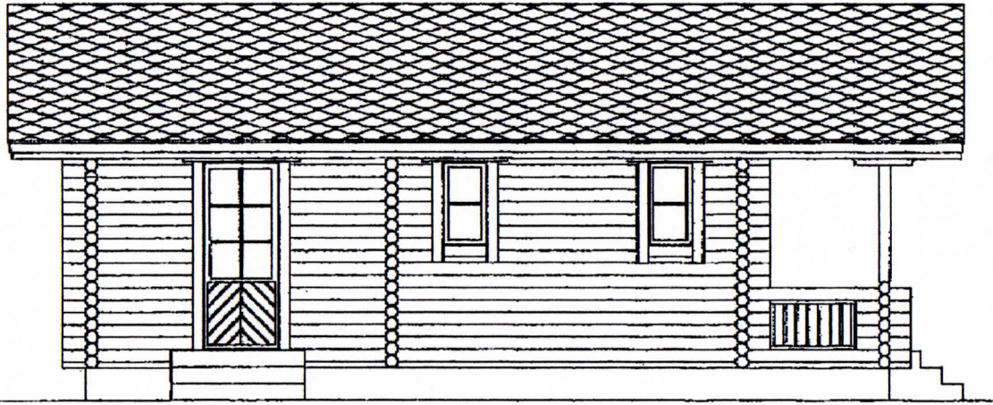
NORTH ELEVATION
