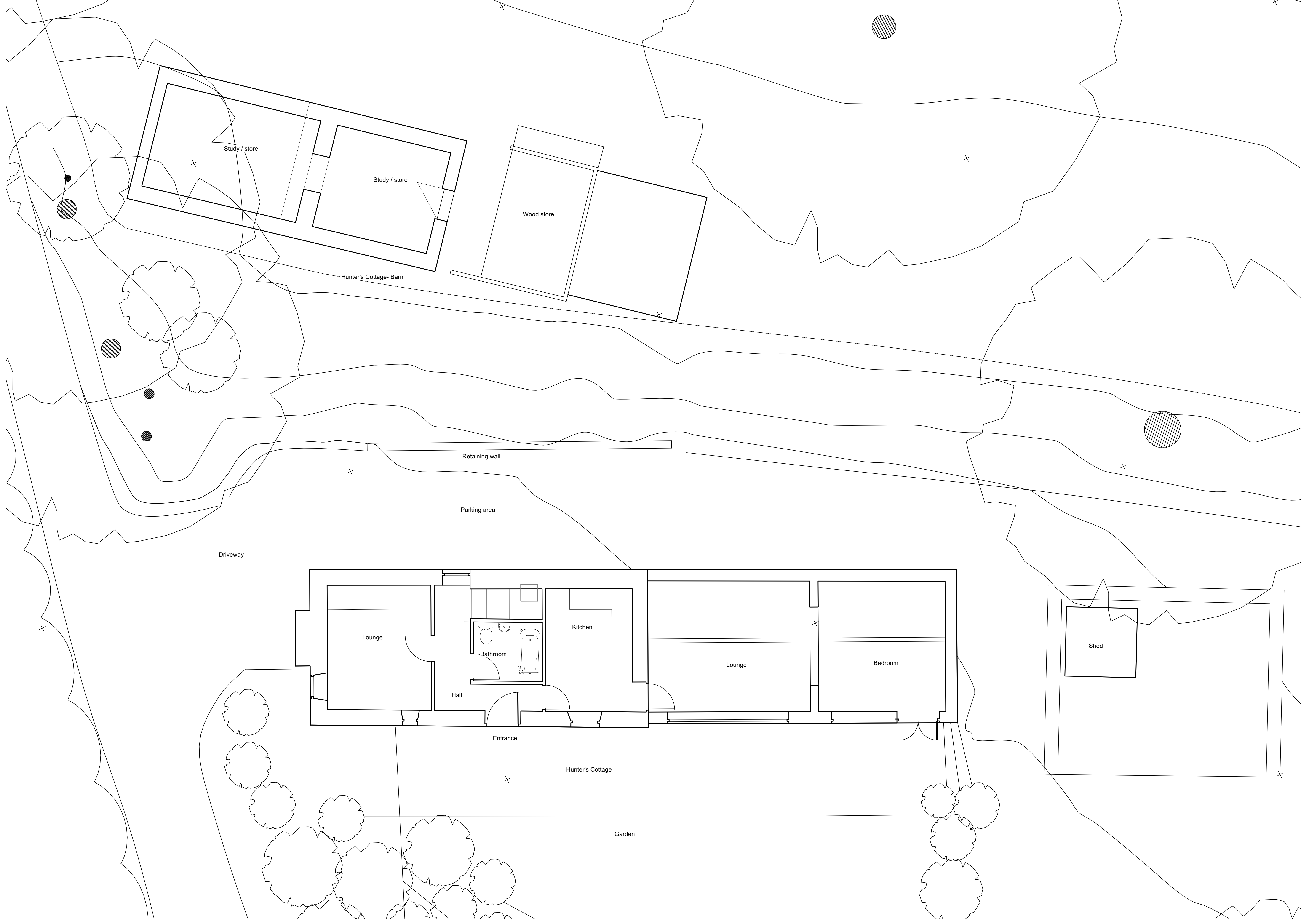
1 Ground floor in Context Scale: 1:50
