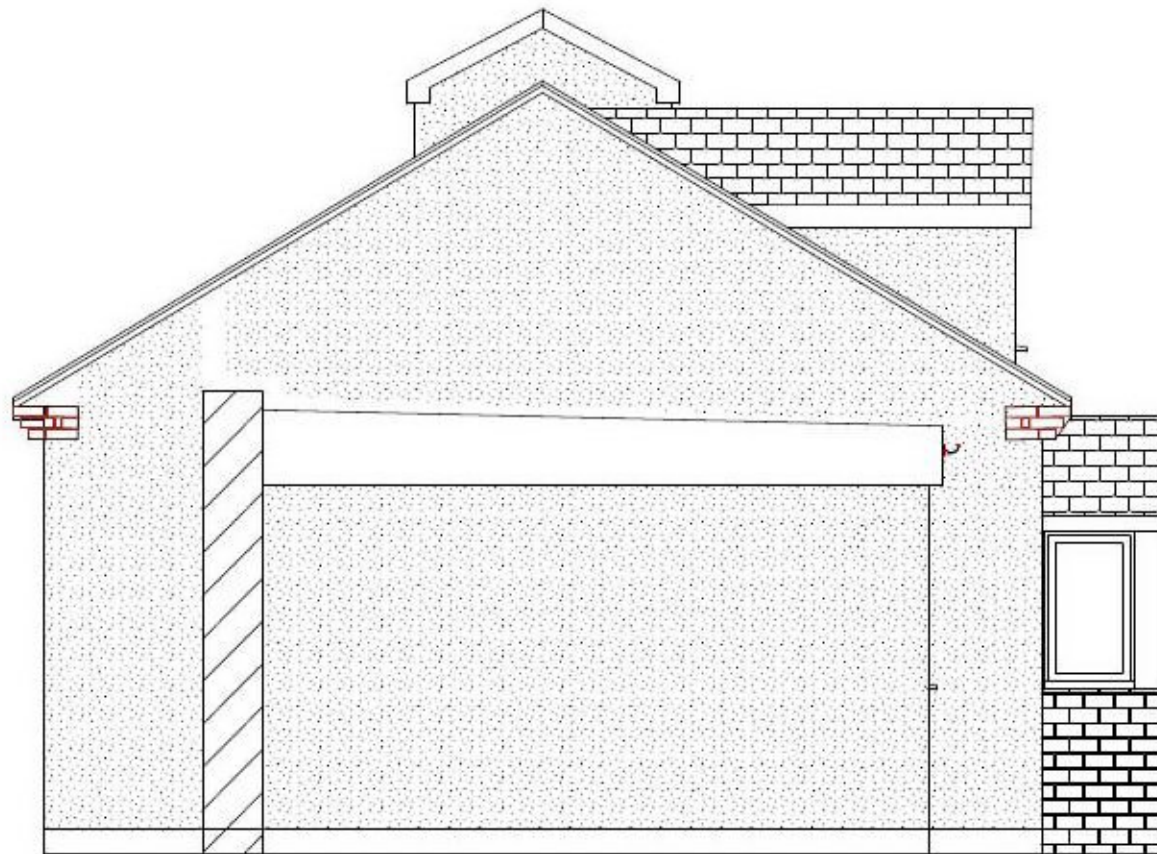
Side Elevation
