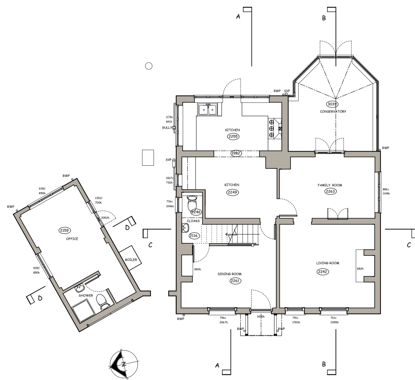
SURVEY - GROUND FLOOR PLAN SCALE 1/100
