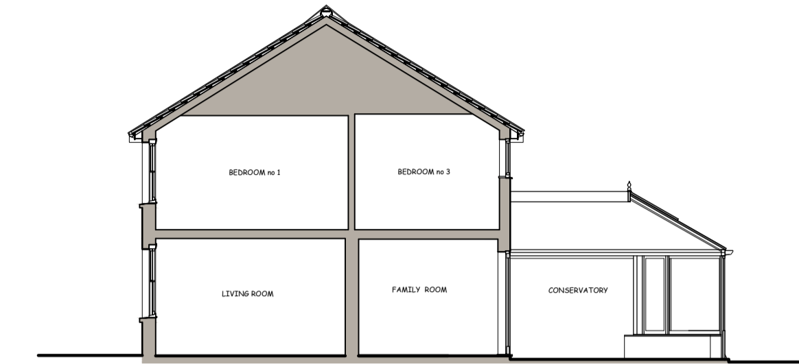
SURVEY - SECTION B-B SCALE 1/100
