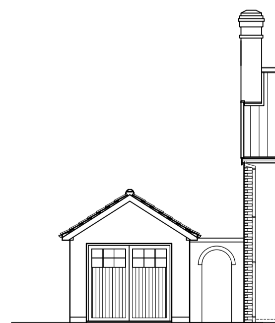
SURVEY - WEST ELEVATION SCALE 1/100
