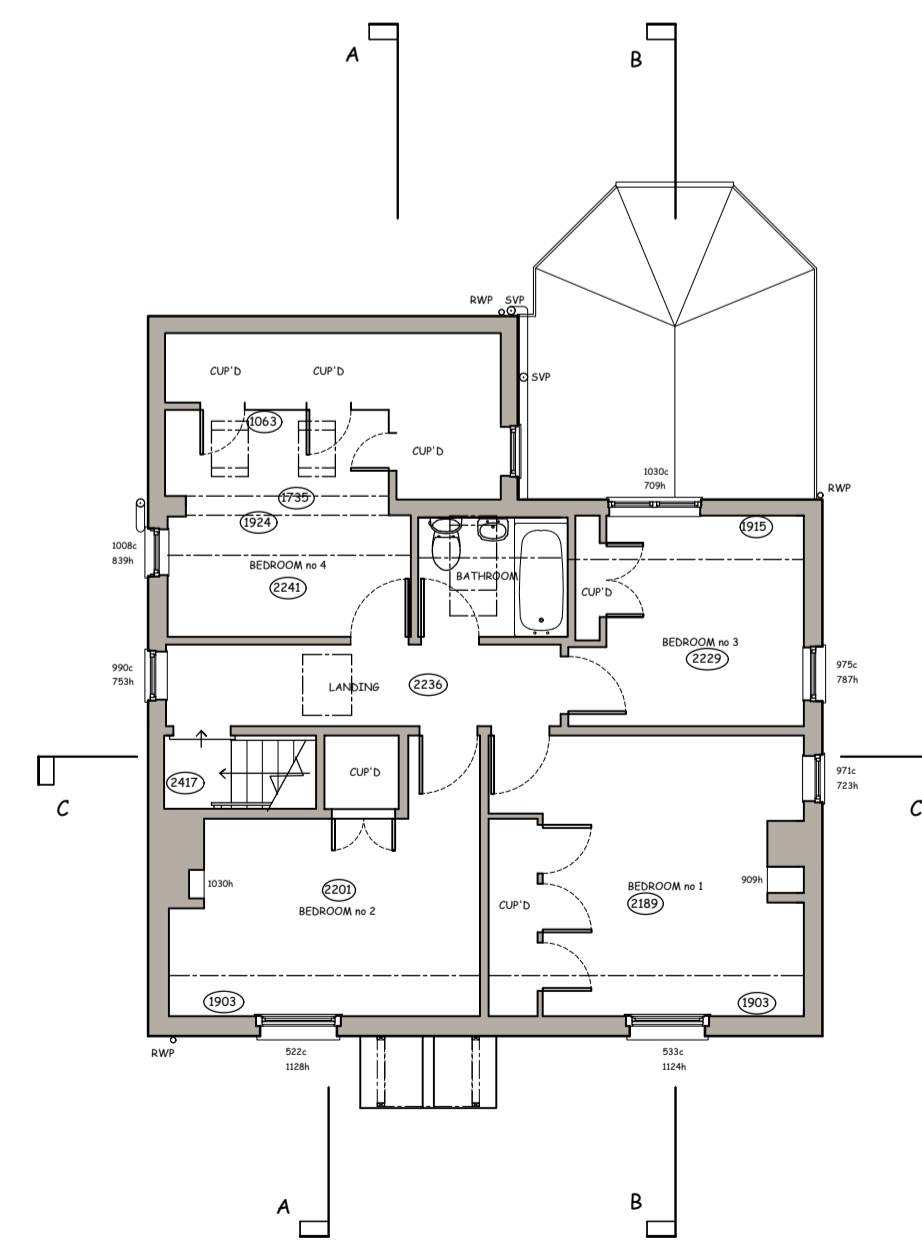
SURVEY - FIRST FLOOR PLAN SCALE 1/100
