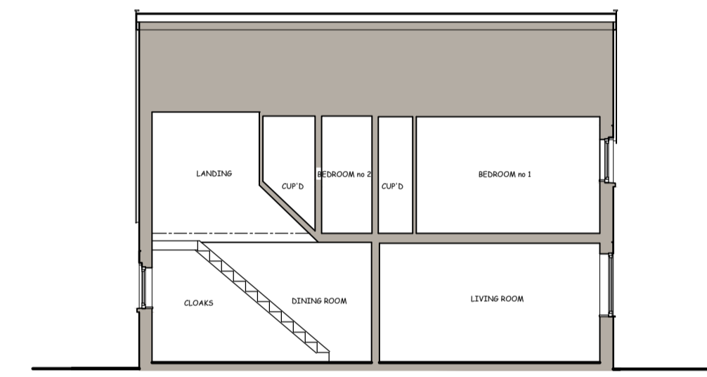
SURVEY - SECTION C-C SCALE 1/100
