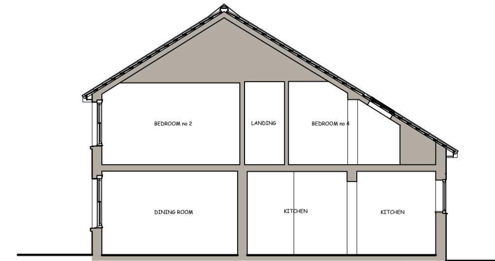
SURVEY - SECTION A-A SCALE 1/100
