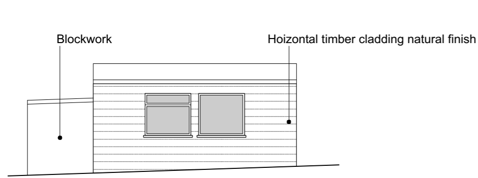
29.00 North Elevation
