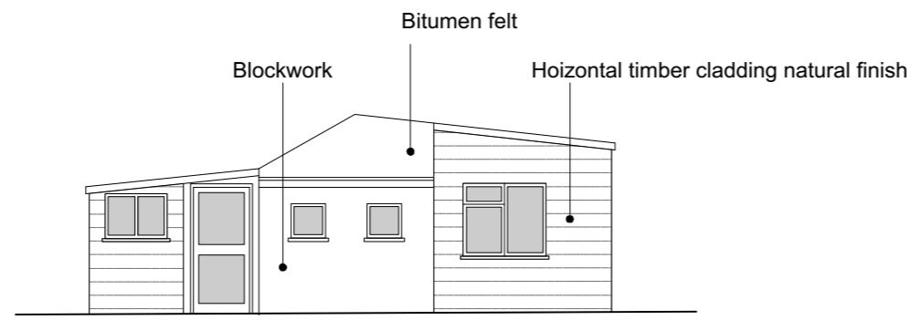
29.00 East Elevation
