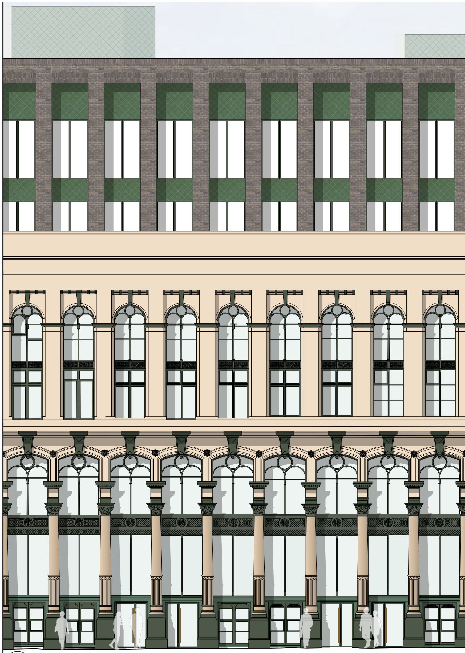
1 Bay Study - Front elevation middle entrances Scale: 1:100
