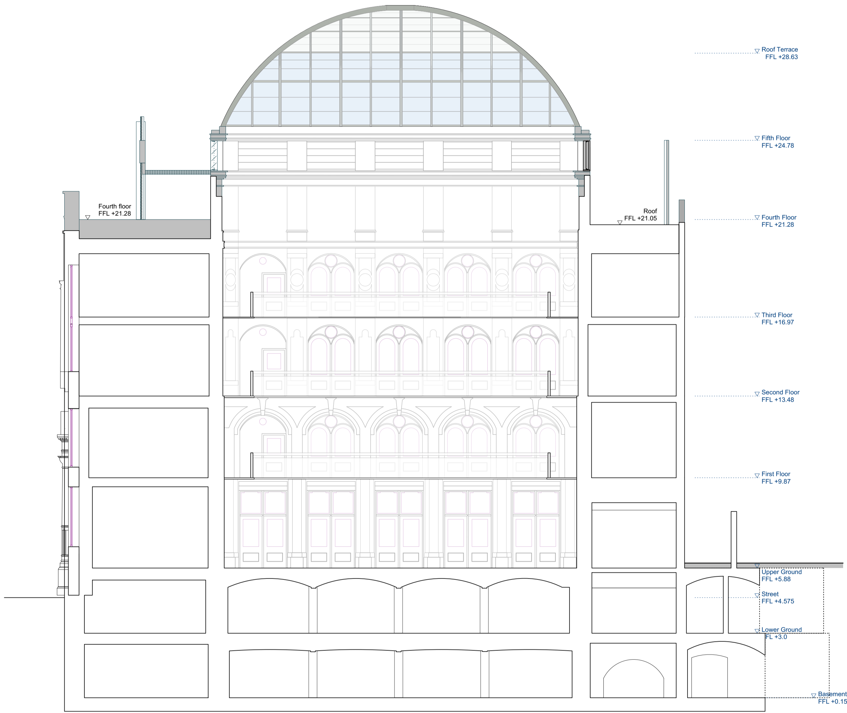
PROPOSED SHORT SECTION B-B
