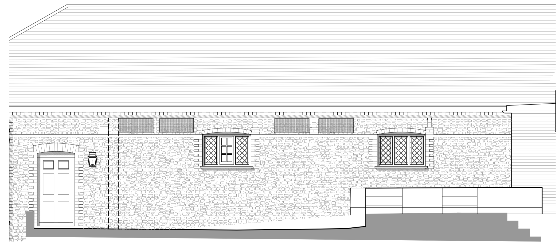
EXTERNAL VIEW OF SUPPLY INTAKE @ B - B
