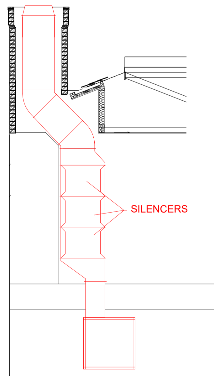
SIDE VIEW OF EXTRACT DUCT @ A - A
