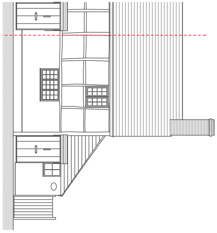
East Elevation 1:50 @ A1
